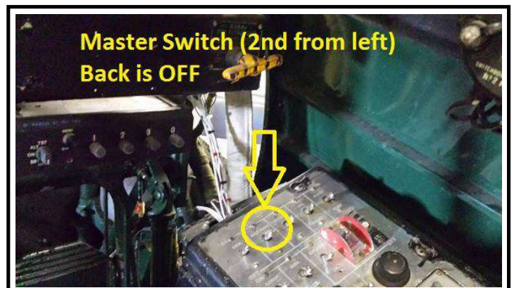
Master (Battery) Switch Front Cockpit, Starboard Side (2 nd from left, looking forward) Back is OFF.
